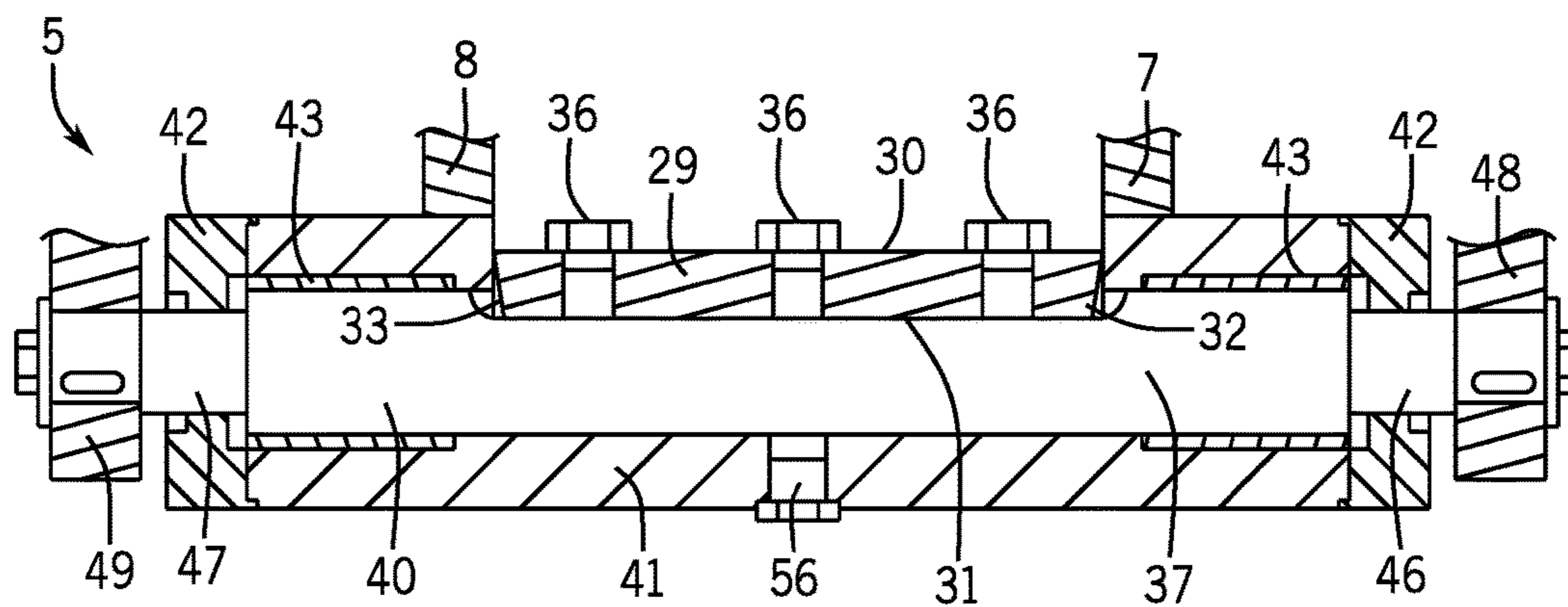
FIG. 6 PRIOR ART
