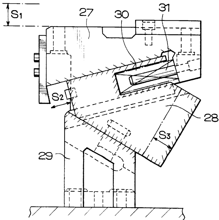
FIG. 6 PRIOR ART
