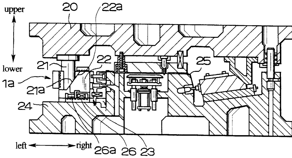
FIG. 5 PRIOR ART
