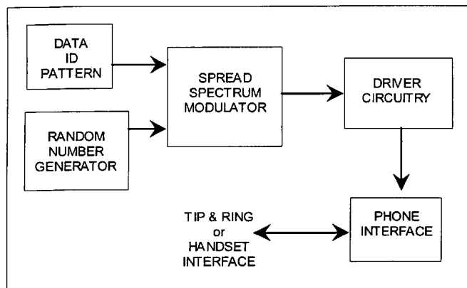
Simplified Invention Block Diagram
