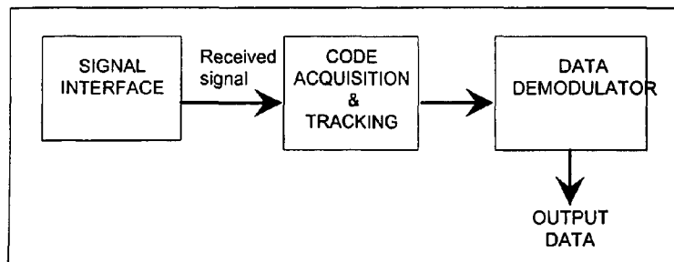
FIGURE 3 - Receiver Block Diagram
