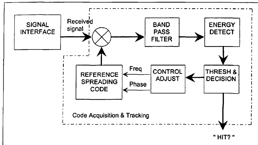
FIGURE 4 - Code Acquisition and Tracking Block Diagram
